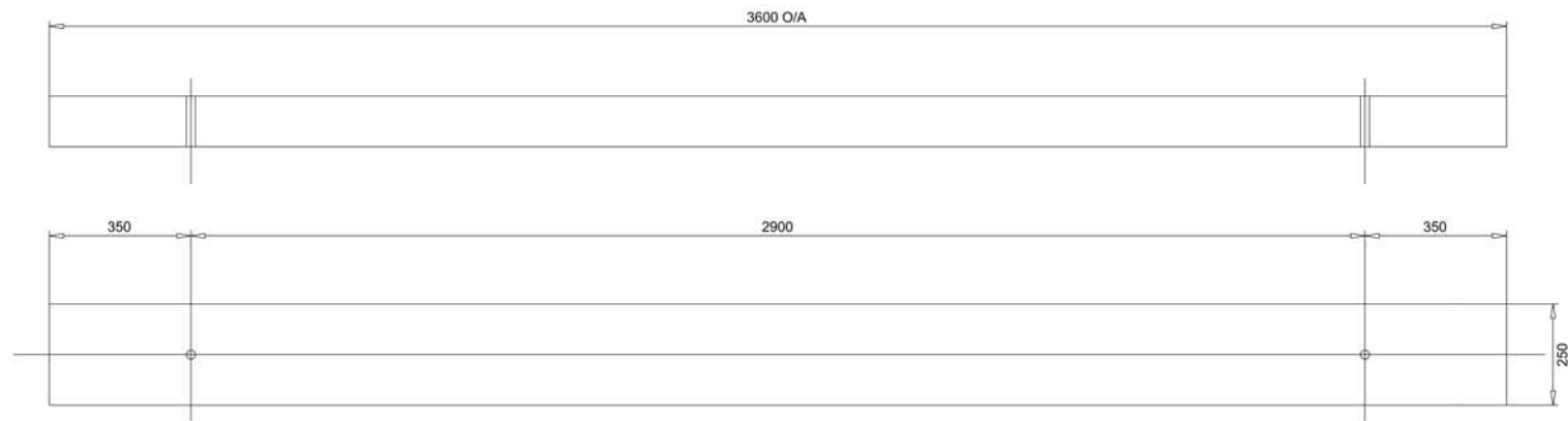
ITEM 8 3600 x 250 x 125 WOOD BAULK SCALE :- 1 : 10
